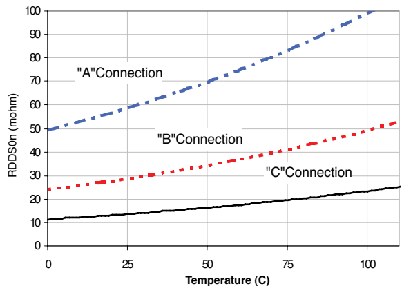
Figure 4. Typical Normalized On-Resistance
