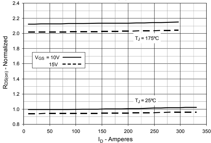
Fig. 5. Normalized R_{DS(on)} vs. Drain Current
