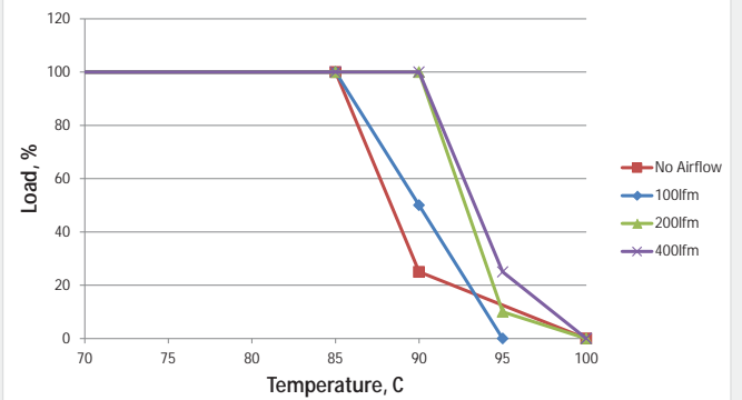
MTC1S2403MC- 24Vin
