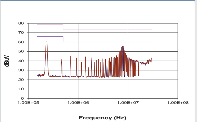
MTC1S2412MC
